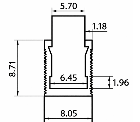
Profile Dimensions:
